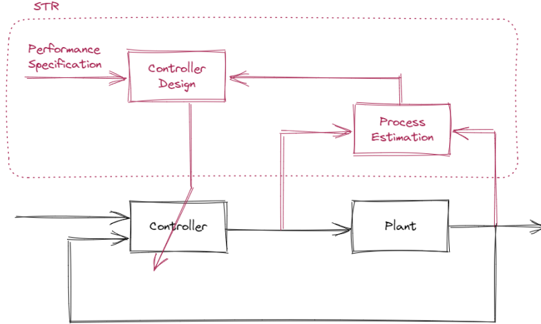
FIGURE 7.4: STR schema.
